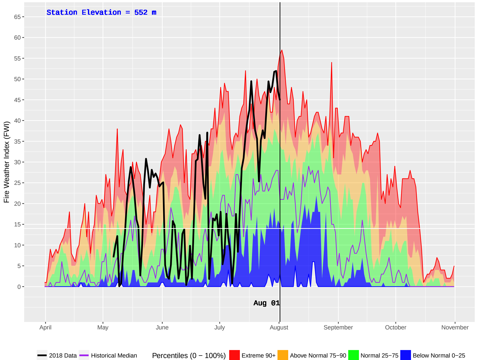
NAHATLATCH (316) : Historical (2001–2016) and Current (2018) Daily Fire Weather Index (FWI)
