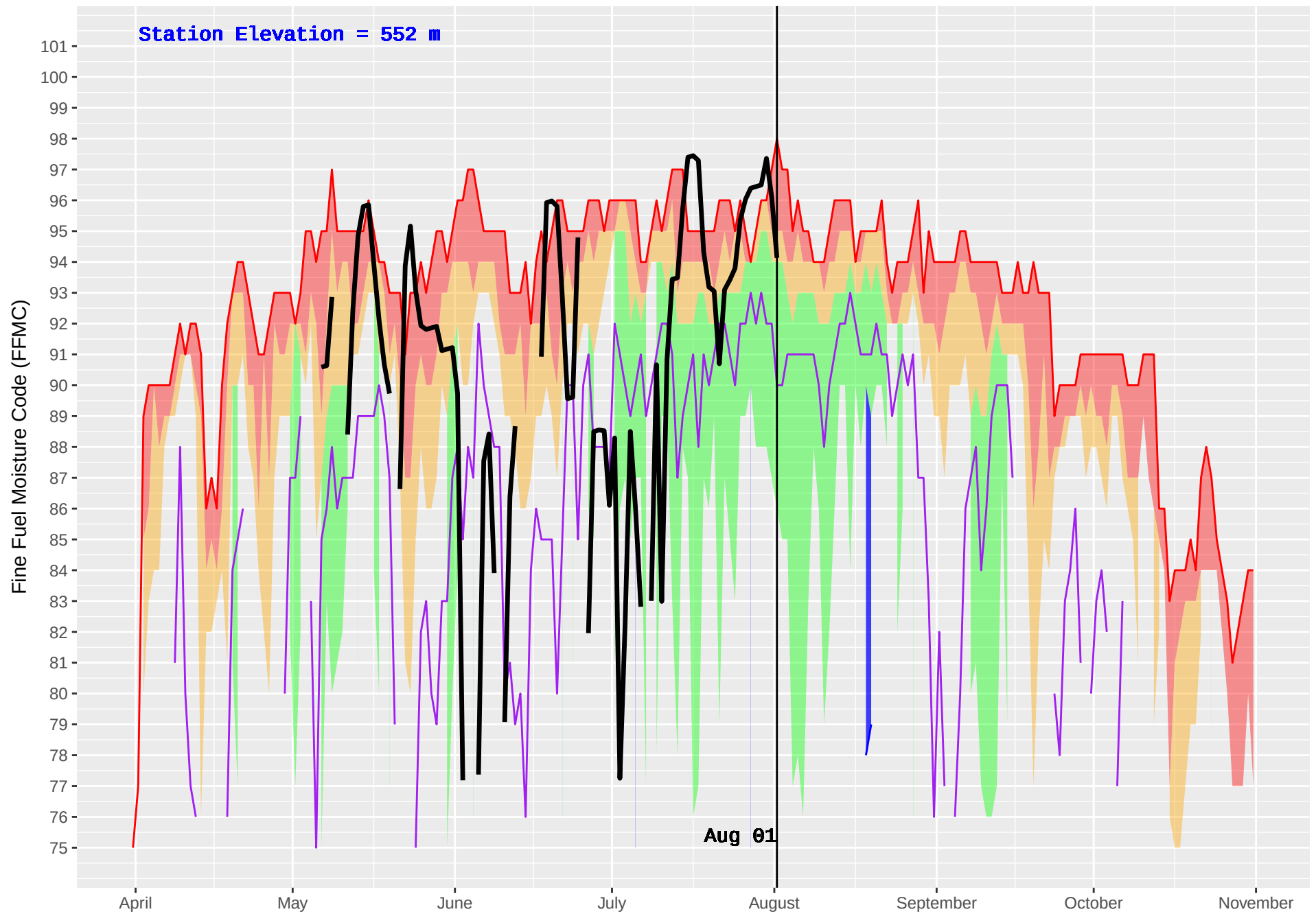
NAHATLATCH (316) : Historical (2001–2016) and Current (2018) Daily Fine Fuel Moisture Code (FFMC)
